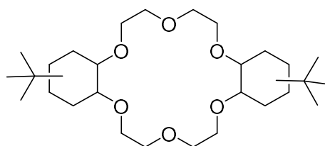
Di-tert-butylidicyclohexano-18-crown-6
