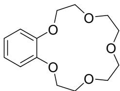
Benzo-15-crown-5
