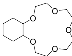
Cyclohexano-15-crown-5
