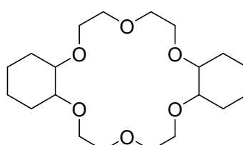
Dicyclohexano-18-crown-6
